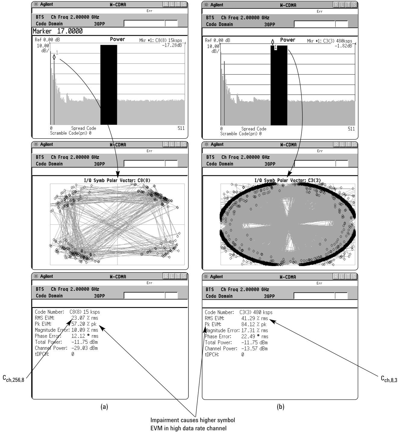
Figure 28. Code domain power measurement of a W CDMA DL signal with the P CCPCH/SCH, CPICH, and two DPCHs (C ch,256,8 and C ch,8,3 ). (a) Symbol EVM for the DPCH at 15 kbps (C ch,256,8 ). (b) Symbol EVM for the DPCH at 480 kbps (C ch,8,3 ).
