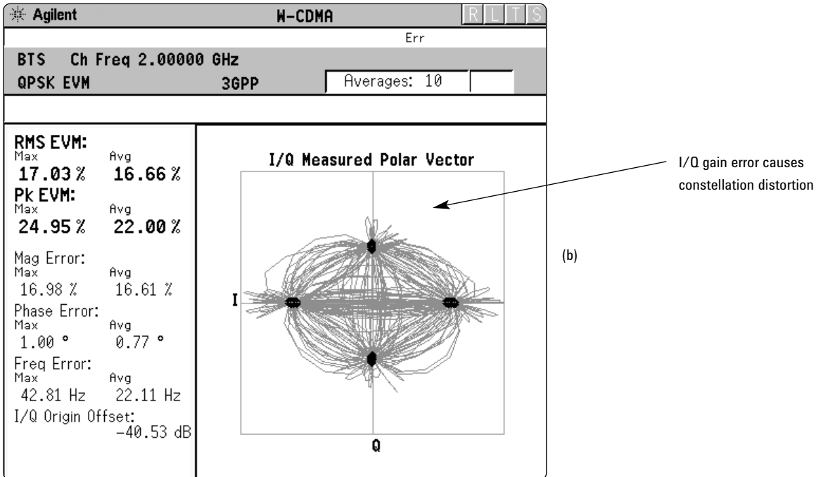
Figure 19. Vector diagram and QPSK EVM measurement for a W CDMA DL signal with a single DPCH. (a) Transmitter without any impairment. (b) Transmitter with an I/Q gain error.
