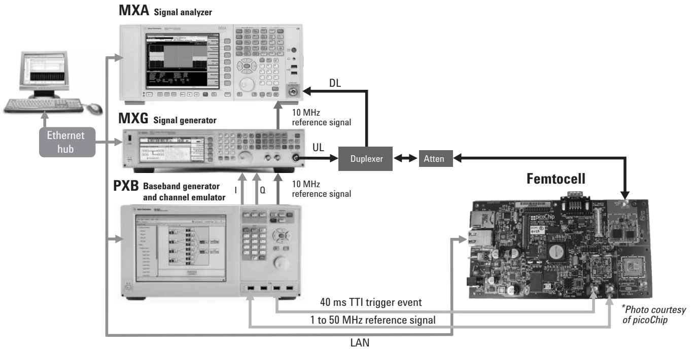
Figure 40. Example of femtocell Tx/Rx RF test setup for R&D
